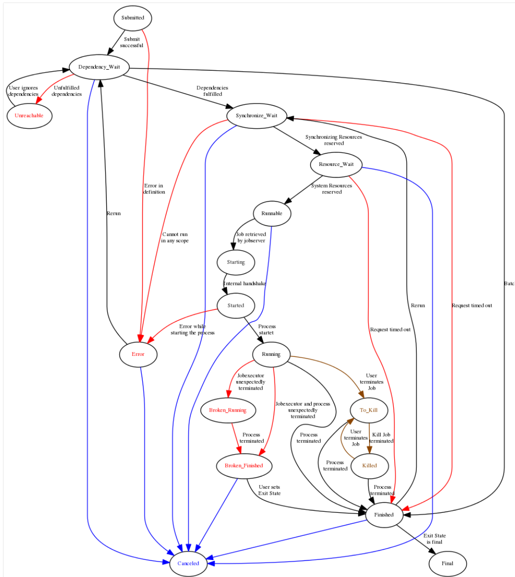
Figure 23.3: State chart for batches and jobs
