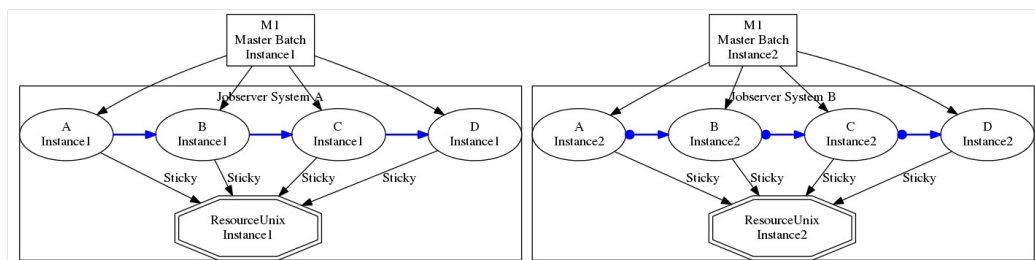
Figure 15.28: Example of load distribution with Sticky Handling
