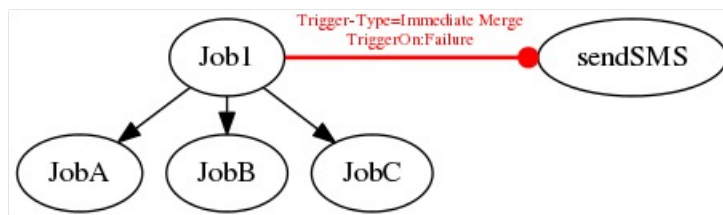
Figure 15.36: Example of an Immediate Merge trigger
