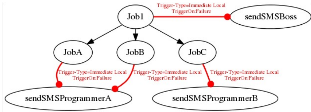
Figure 15.37: Example of an Immediate Local trigger
