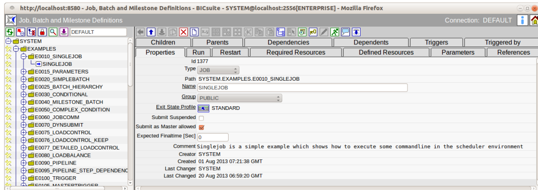
Figure 15.9: Job Definition properties
