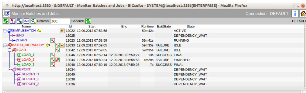
Figure 23.1: Search Running Jobs
