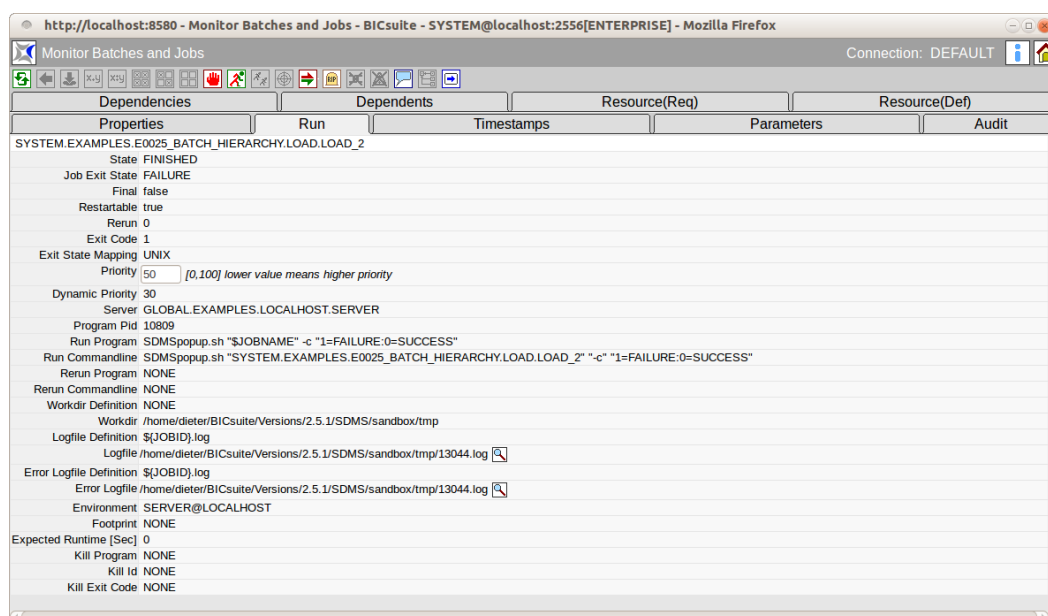
Figure 22.7: Details mask for jobs
