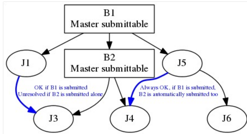
Figure 15.23: Example for Unresolved Handling
