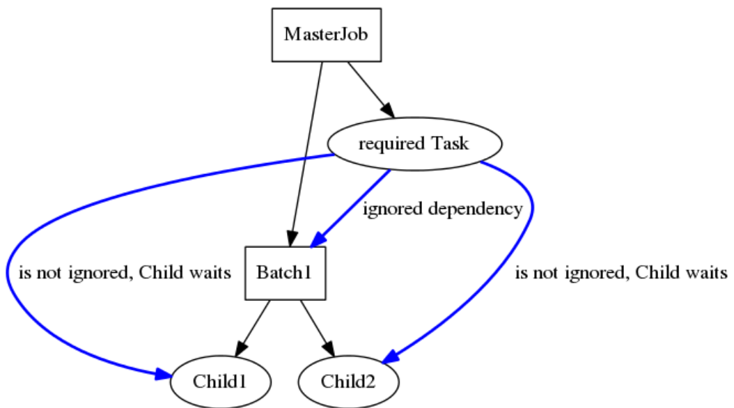
Figure 22.14: Example of a Recursive Ignore
