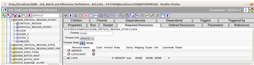
Figure 15.25: Jobs; Required Resources tab
