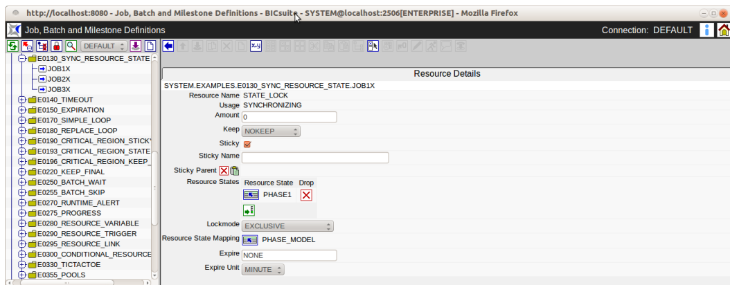
Figure 15.26: Batches and Jobs; Resource Requirement details
