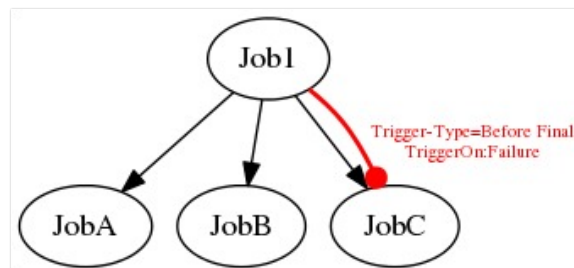
Figure 15.38: Example of a Before Final Trigger
