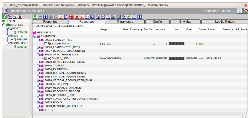
Figure 14.1: Job servers and resources
