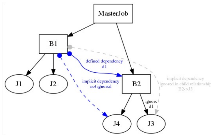
Figure 15.18: Example of Ignored Dependencies
