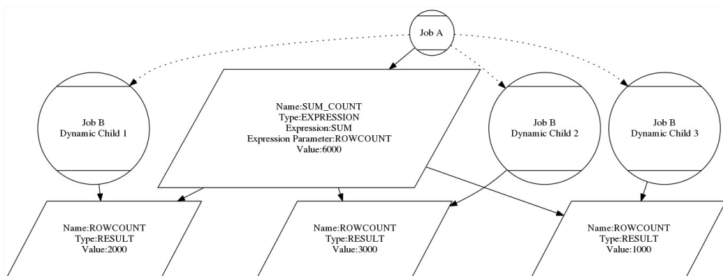
Figure 15.32: Example using Expression parameters
