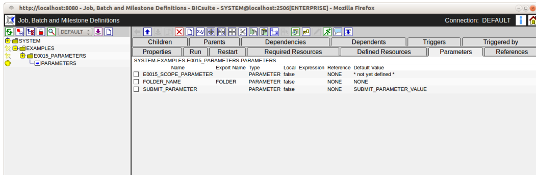
Figure 15.30: Batches and Jobs; Parameters tab
