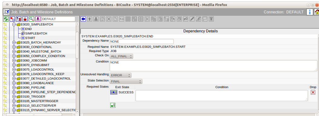
Figure 15.22: Batches and Jobs; Dependency Details
