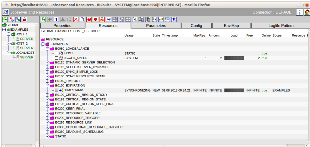
Figure 14.2: Job servers and Scope Navigator
