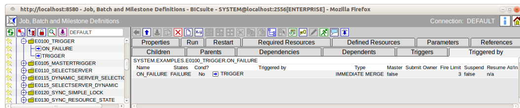
Figure 15.41: Jobs and batches; Triggered By tab
