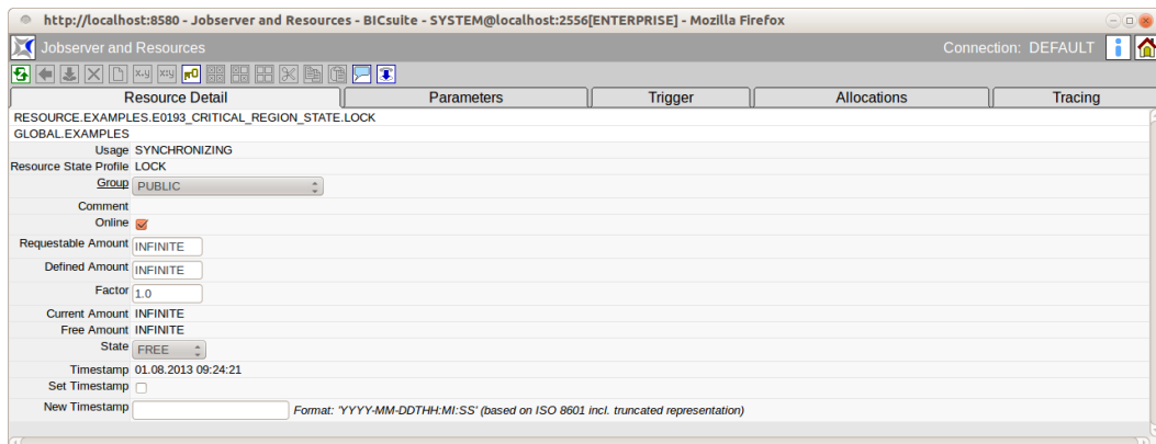
Figure 14.6: Resource Details
