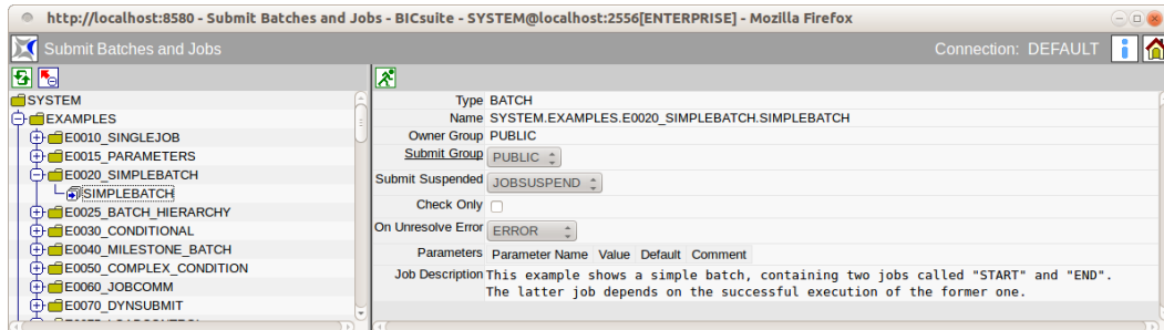
Figure 20.2: Submit navigation
