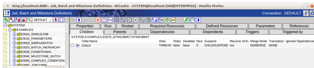
Figure 15.14: Batches and Jobs; Children tab
