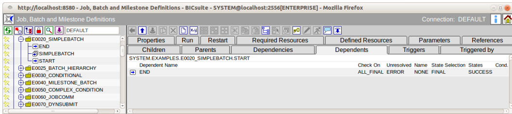
Figure 15.24: Batches and Jobs; Dependents tab
