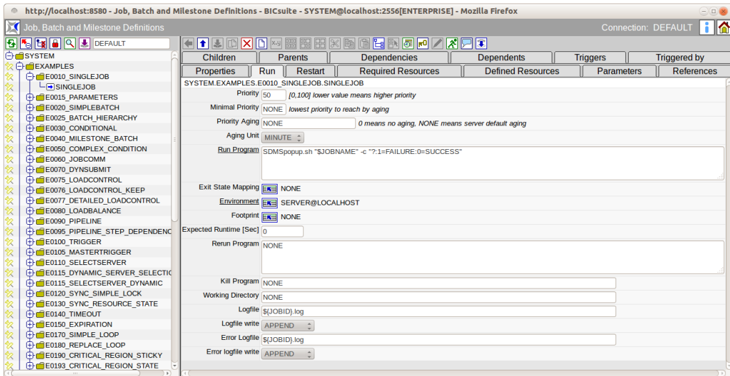
Figure 15.12: Run Job tab
