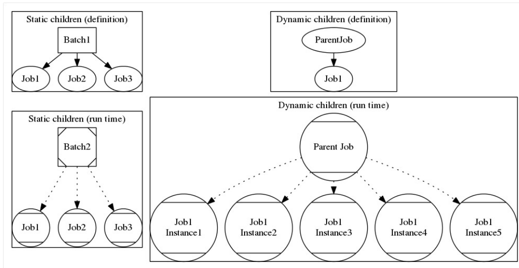
Figure 15.16: Static and dynamic children
