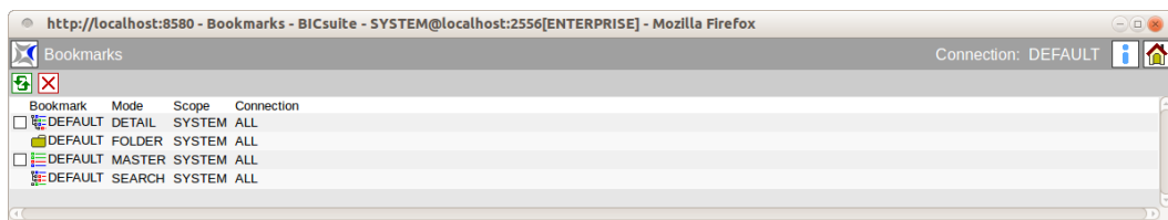
Figure 21.1: Bookmarks
