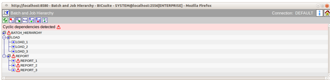
Figure 15.45: Cyclic dependencies
