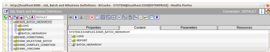
Figure 15.6: Folder content
