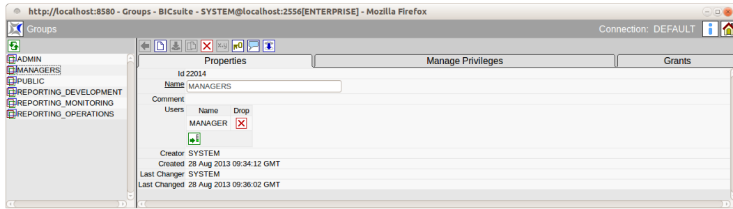
Figure 18.2: Group properties
