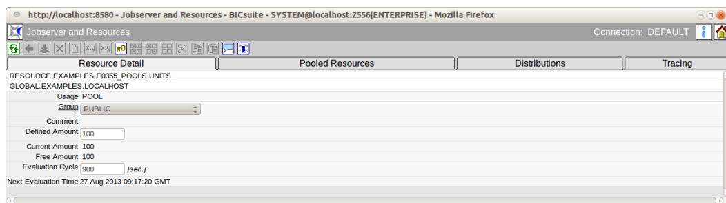
Figure 14.14: Pooled Resources
