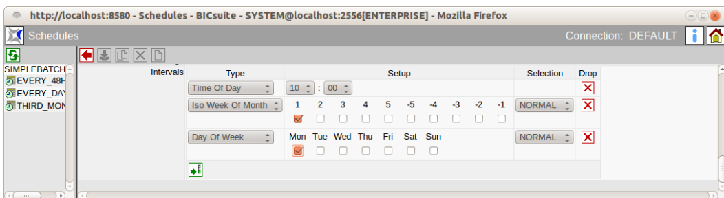
Figure 19.10: ISO Week of Month Filter
