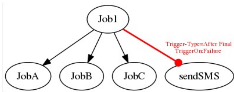
Figure 15.39: Example of an After Final Trigger
