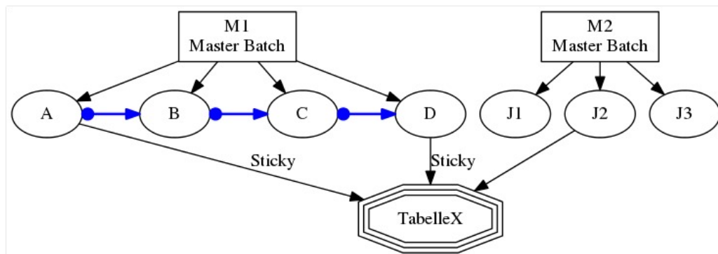
Figure 15.27: Example of Sticky Handling
