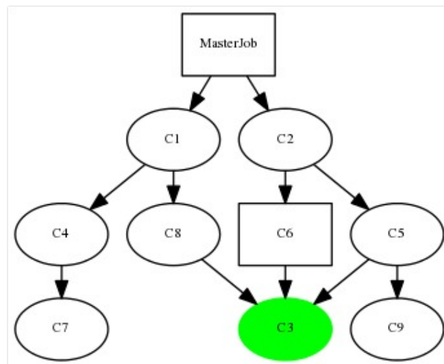
Figure 15.17: Example of Merge Mode
