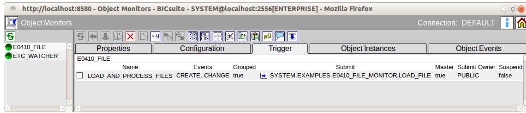
Figure 26.6: Object Monitoring triggers
