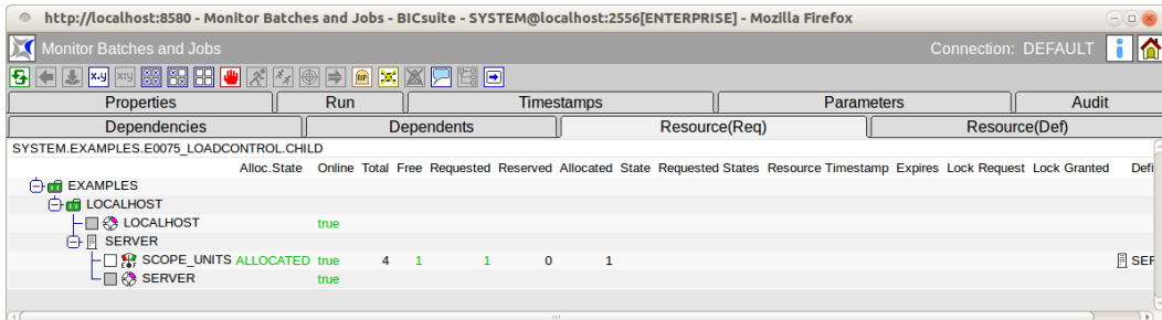
Figure 22.18: Job Resource Requirements
