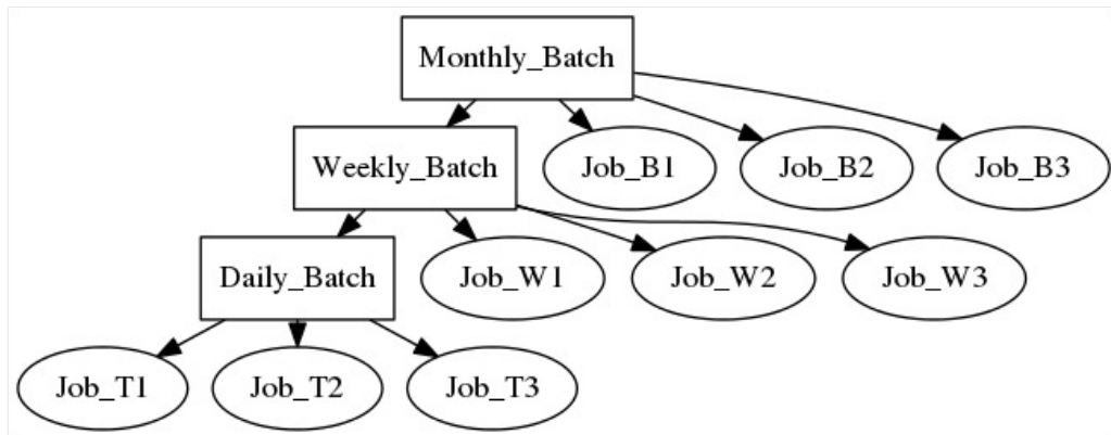
Figure 15.10: Examples of batches
