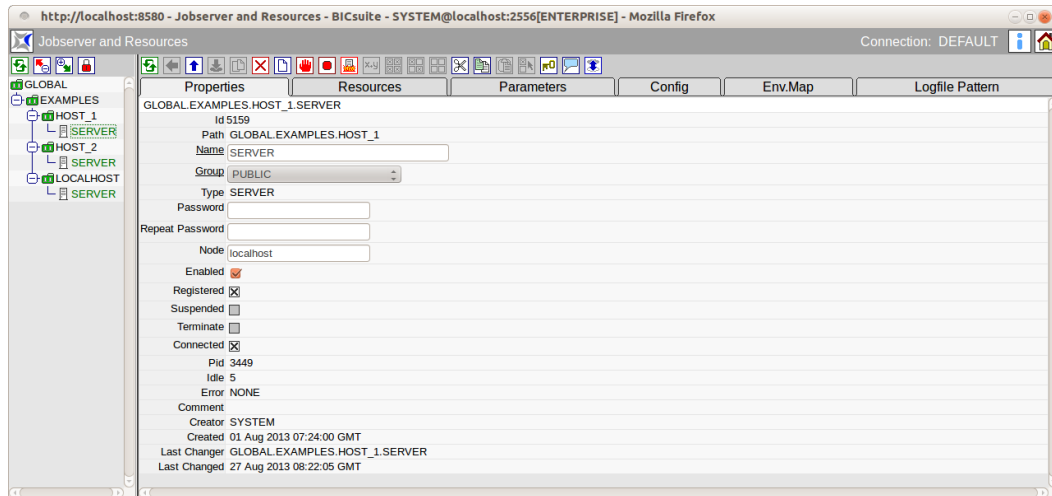
Figure 14.4: Job server properties
