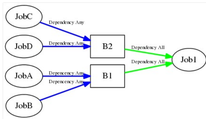
Figure 15.21: Example of Dependency Modes
