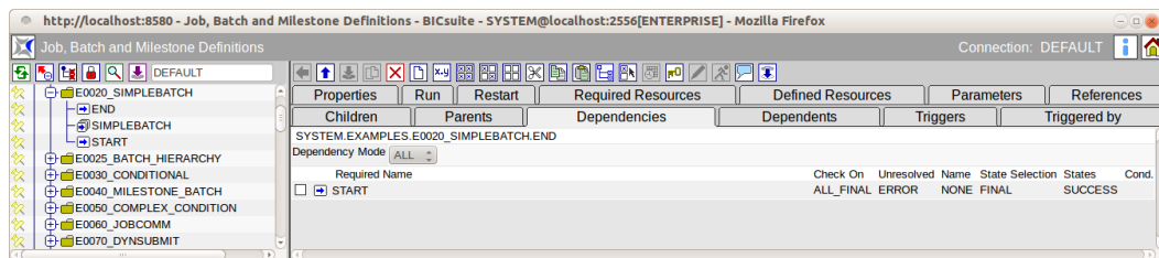
Figure 15.20: Batches and Jobs; Dependencies tab
