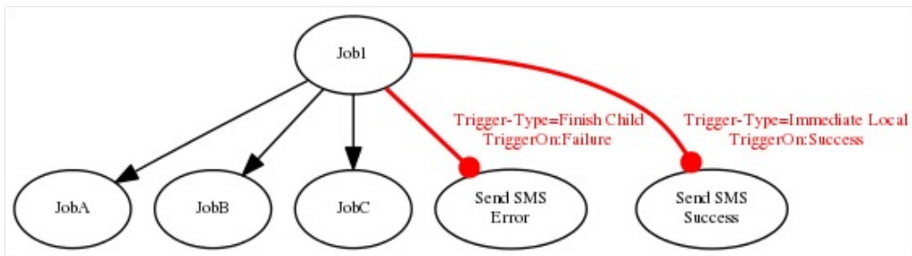
Figure 15.40: Example of a Finish Child Trigger
