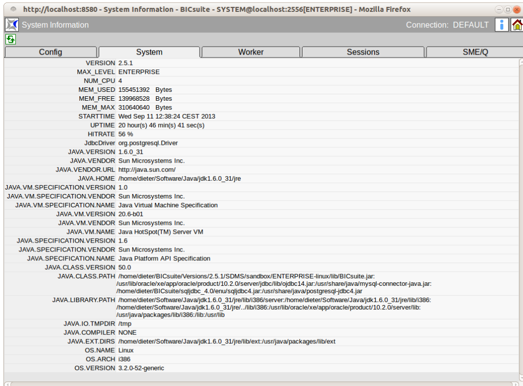
Figure 25.3: System runtime environment
