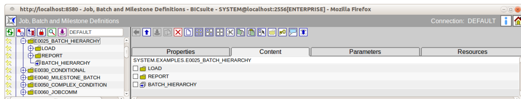
Figure 14.6: Folder content
