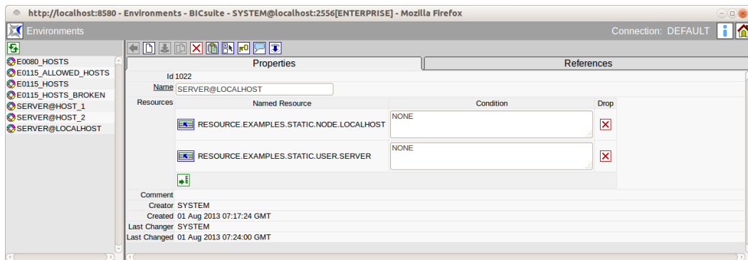
Figure 11.3: Environment properties
