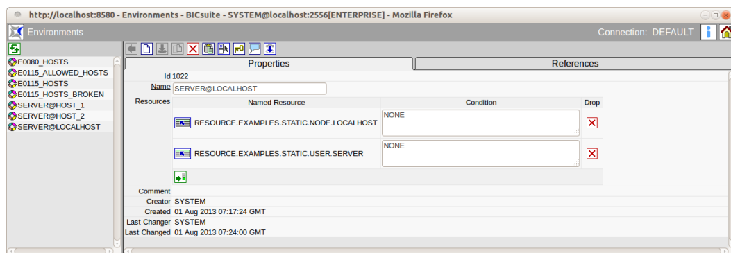
Figure 11.1: Environments
