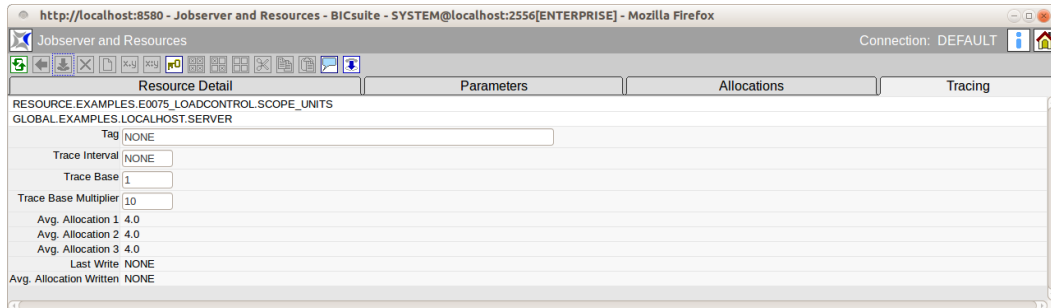
Figure 13.9: Resource Tracing
