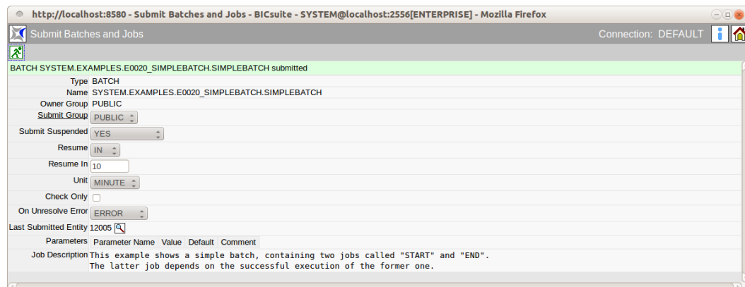
Figure 19.3: Submit editor
