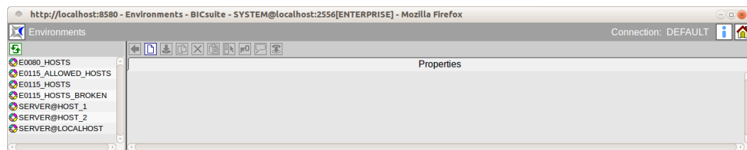
Figure 11.2: Environment navigator
