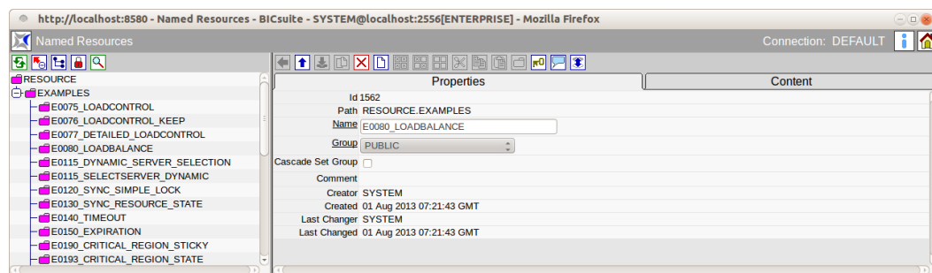
Figure 10.2: Categories; Properties tab
