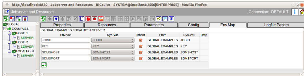
Figure 13.12: Job server environment mapping
