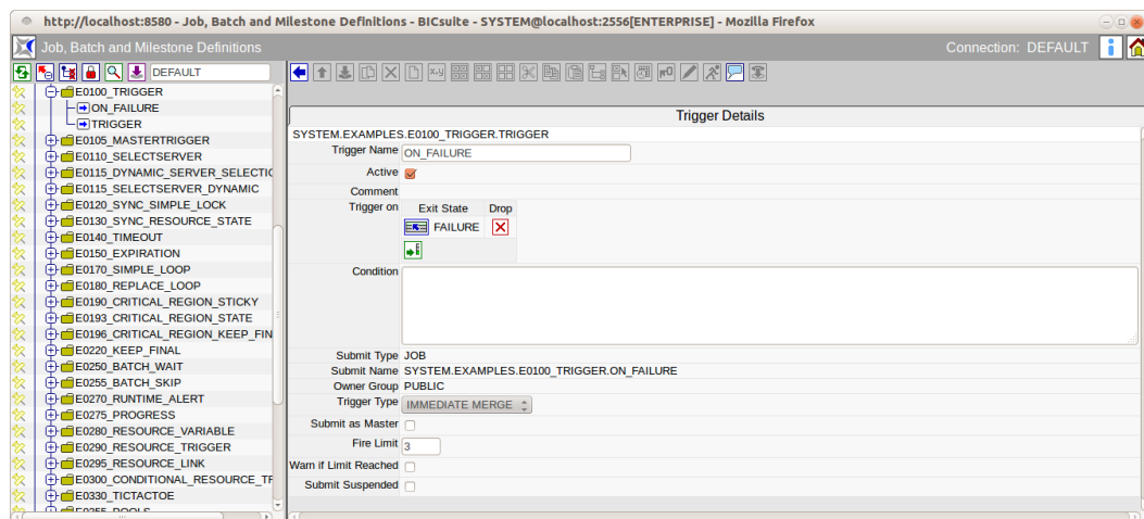
Figure 14.35: Batches and Jobs; Trigger Details tab
