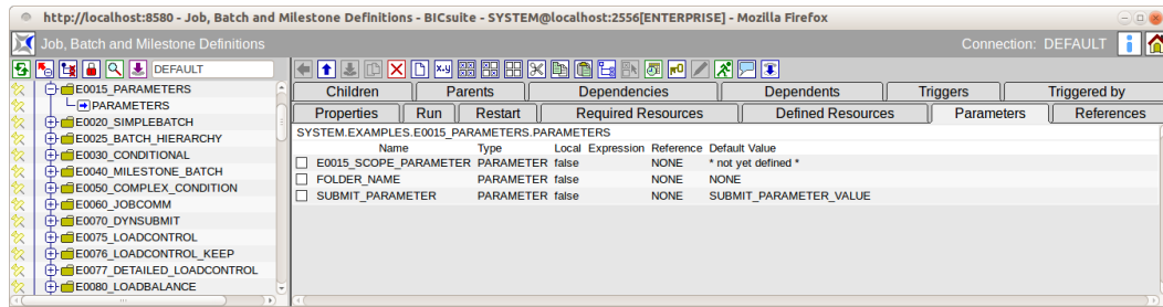
Figure 14.30: Batches and Jobs; Parameters tab
