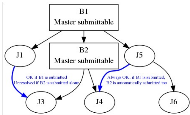
Figure 14.23: Example for Unresolved Handling
