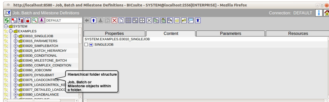
Figure 14.2: Navigator for batches and jobs
