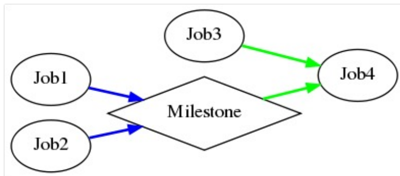
Figure 14.11: Example of a milestone
