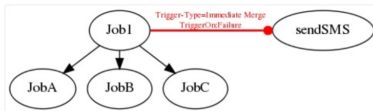
Figure 14.36: Example of an Immediate Merge trigger
