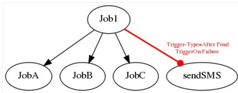
Figure 14.39: Example of an After Final Trigger
