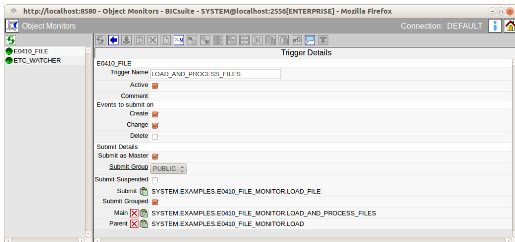
Figure 25.7: Object Monitoring Trigger Details
