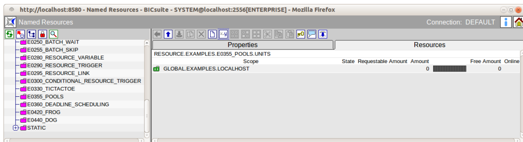
Figure 10.9: Named Resources; Pool properties
