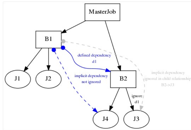
Figure 14.18: Example of Ignored Dependencies
