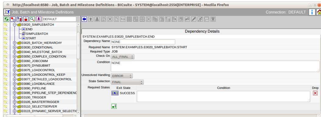
Figure 14.22: Batches and Jobs; Dependency Details
