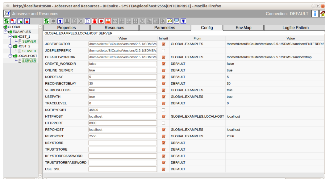
Figure 13.11: Job server and scope configuration
