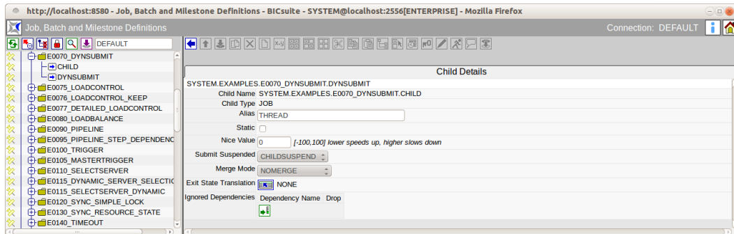
Figure 14.15: Batches and Jobs; Child Details tab
