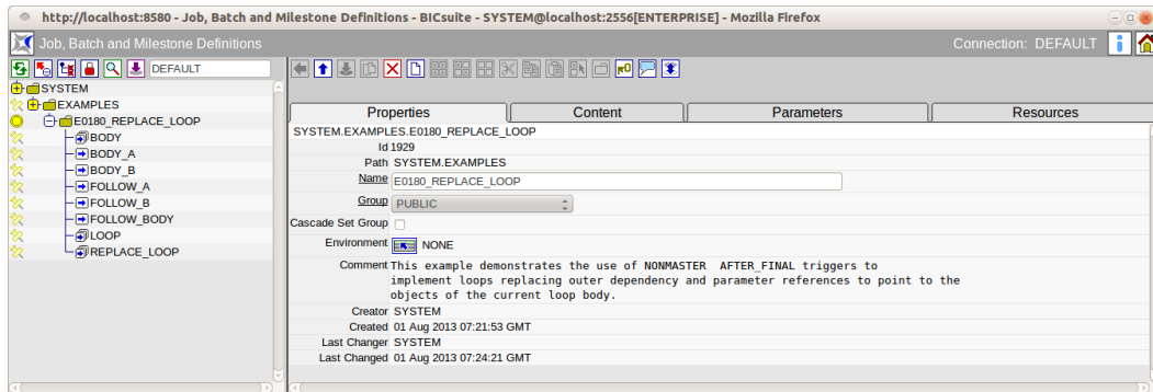
Figure 14.4: Batches and Jobs; view with a pin
