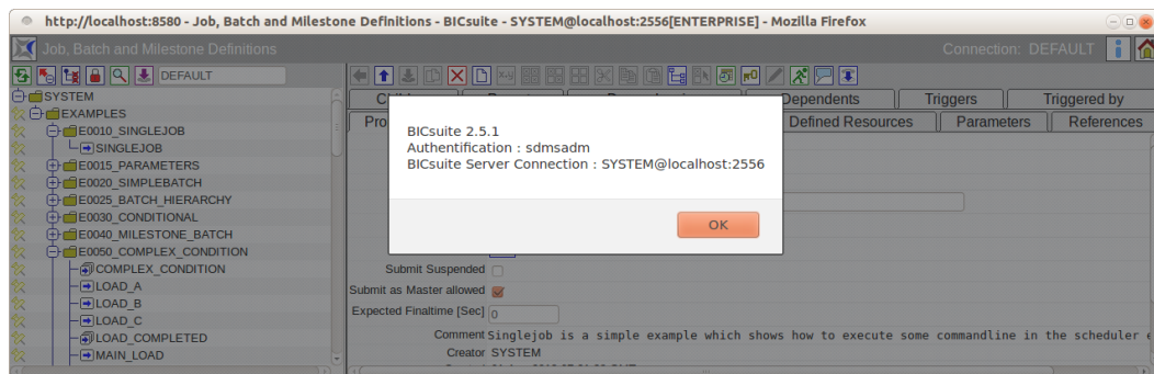
Figure 1.6: About window
