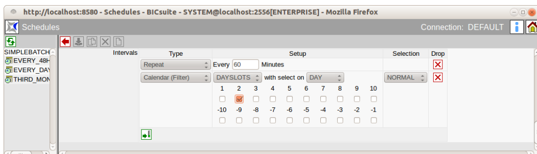
Figure 18.14: Calendar Filter
