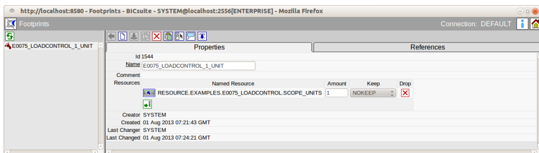
Figure 12.1: Footprints
