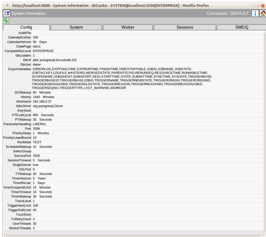
Figure 24.1: System Information
