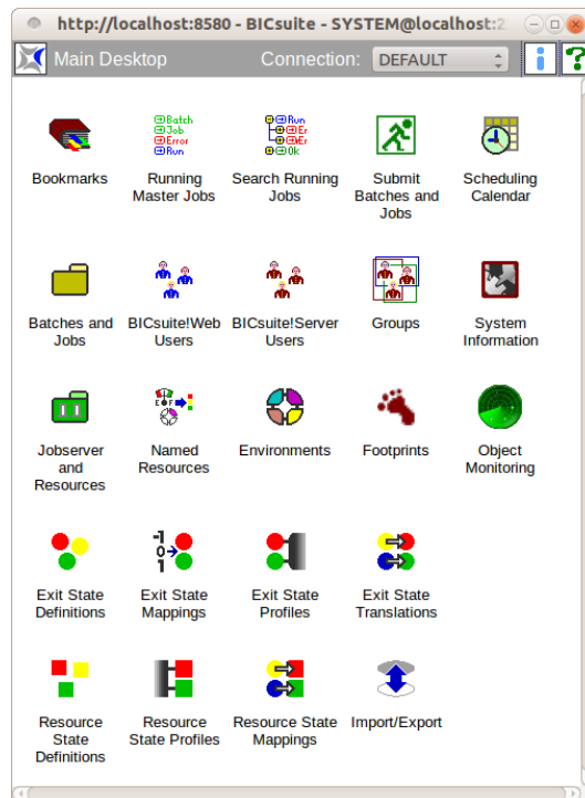
Figure 1.3: Main Desktop
