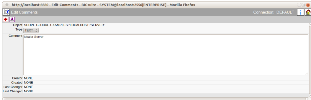
Figure 1.41: Recording comments
