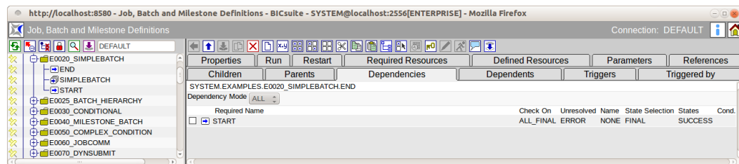
Figure 14.20: Batches and Jobs; Dependencies tab
