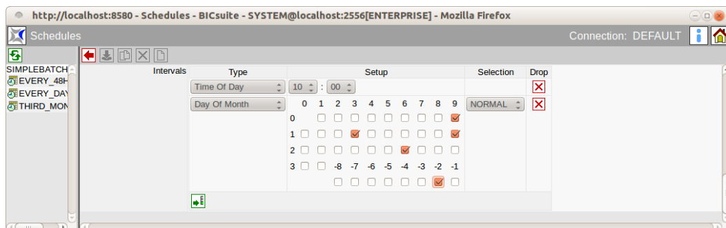
Figure 18.8: Day of Month Filter
