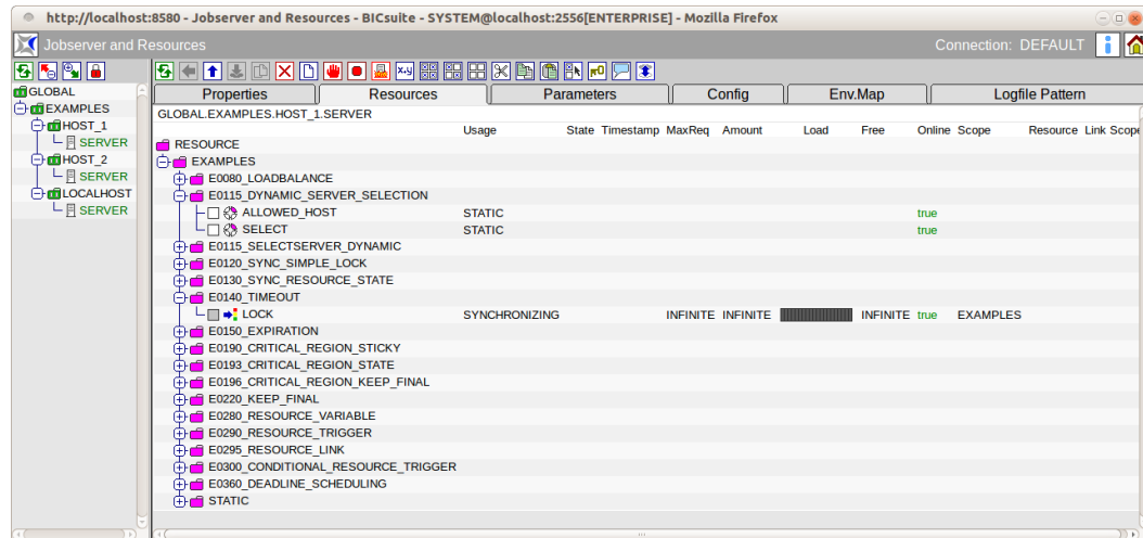
Figure 13.5: Job server and scope resources
