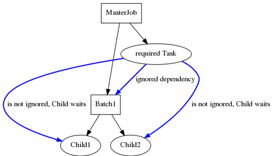
Figure 21.14: Example of a Recursive Ignore
