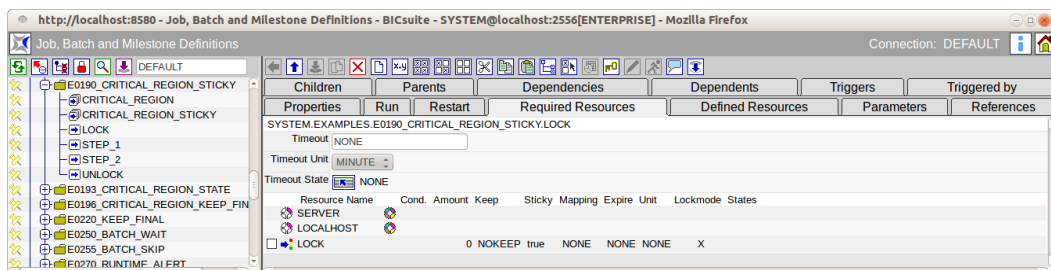
Figure 14.25: Jobs; Required Resources tab
