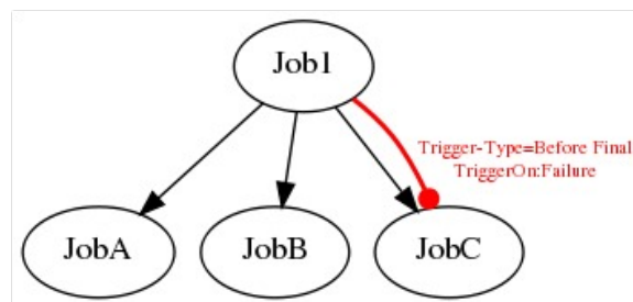
Figure 14.38: Example of a Before Final Trigger
