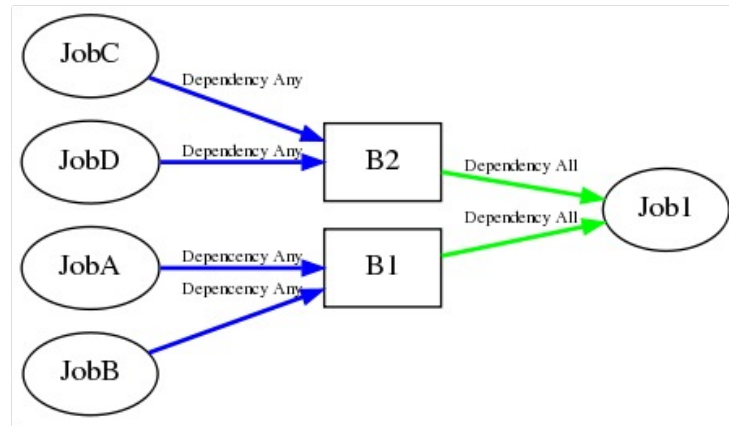
Figure 14.21: Example of Dependency Modes
