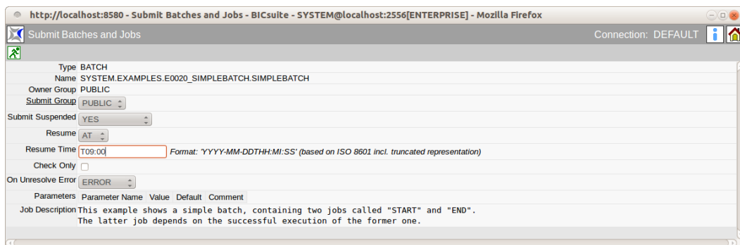
Figure 19.1: Submit Batches and Jobs
