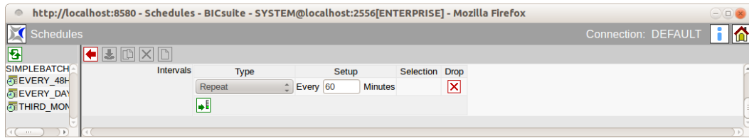
Figure 18.4: Repeat Driver
