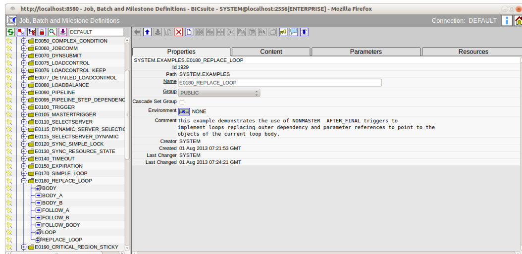
Figure 14.5: Folder properties
