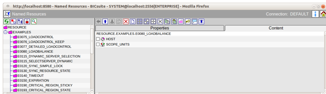
Figure 10.1: Named Resources
