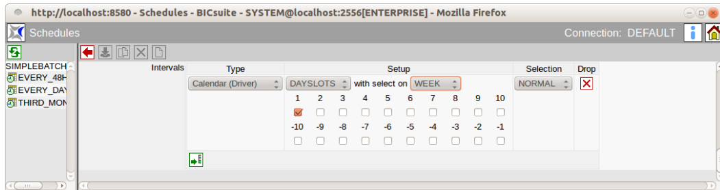
Figure 18.13: Calendar Driver
