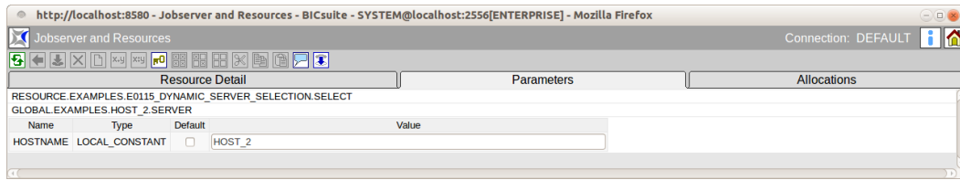
Figure 13.7: Resource parameters
