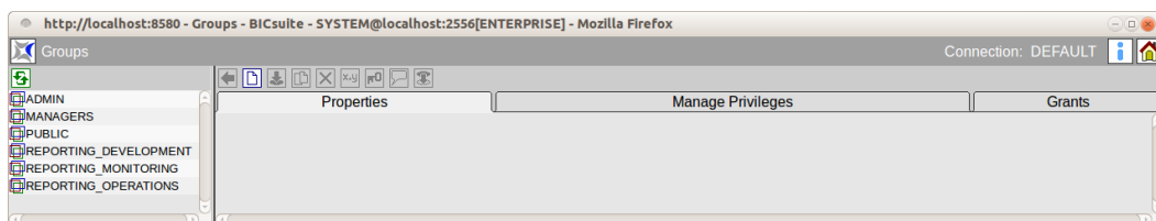
Figure 17.1: Group management
