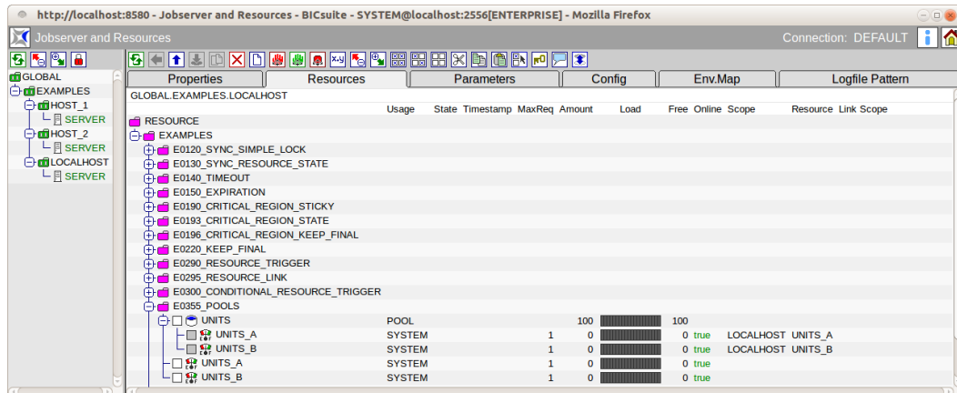
Figure 13.14: Pooled Resources
