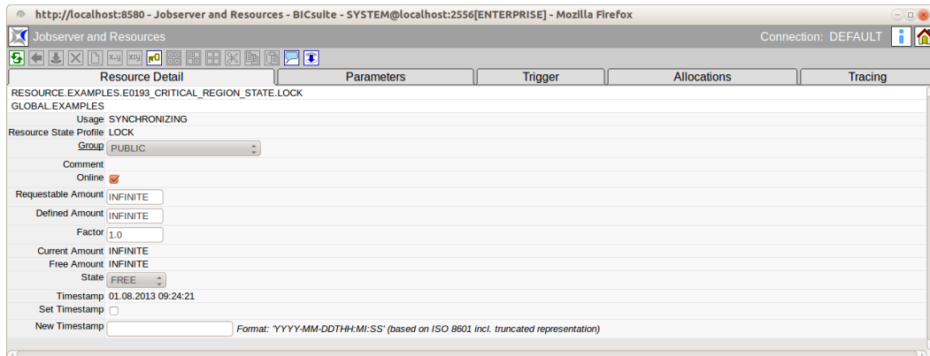
Figure 13.6: Resource Details
