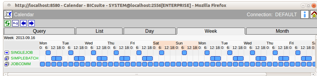
Figure 23.5: Calendar Week tab
