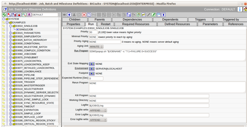
Figure 14.12: Run Job tab
