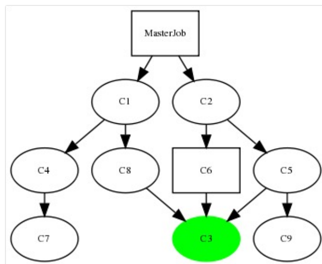
Figure 14.17: Example of Merge Mode
