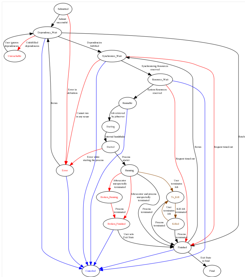
Figure 21.3: State chart for batches and jobs
