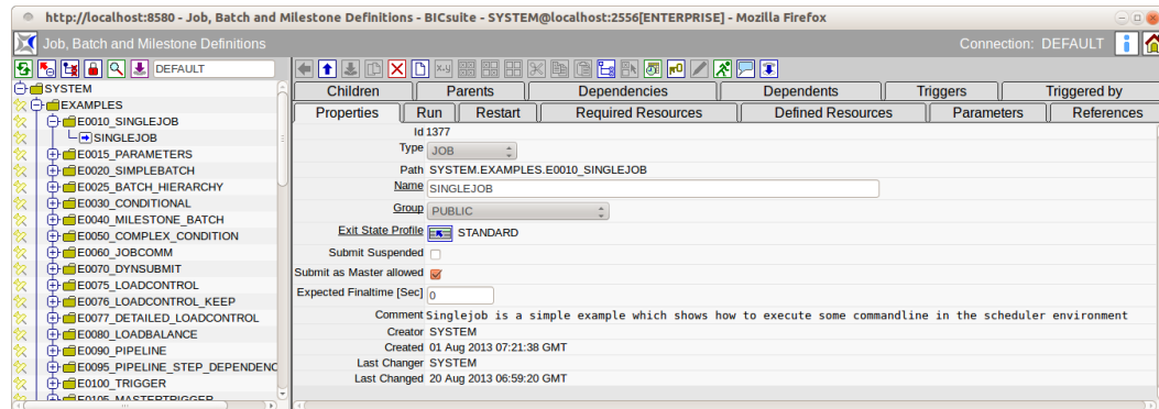
Figure 14.9: Job Definition properties
