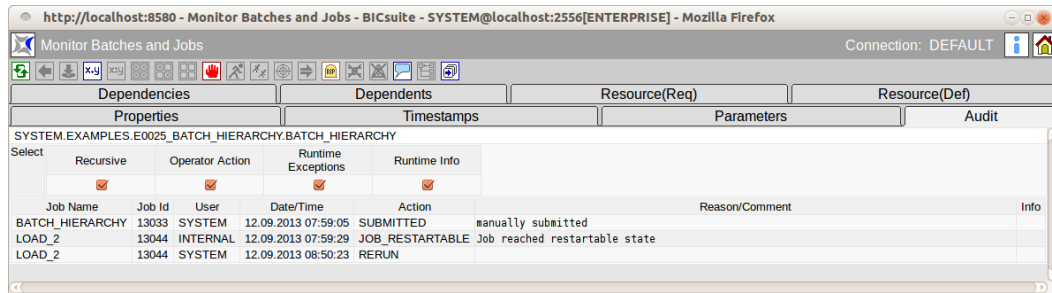
Figure 21.22: Batch and job auditing
