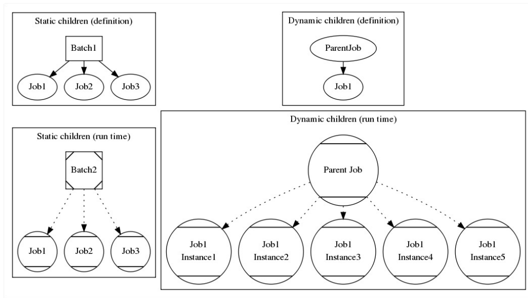
Figure 14.16: Static and dynamic children
