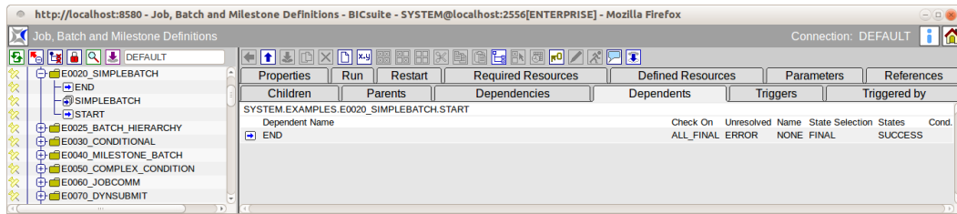
Figure 14.24: Batches and Jobs; Dependents tab
