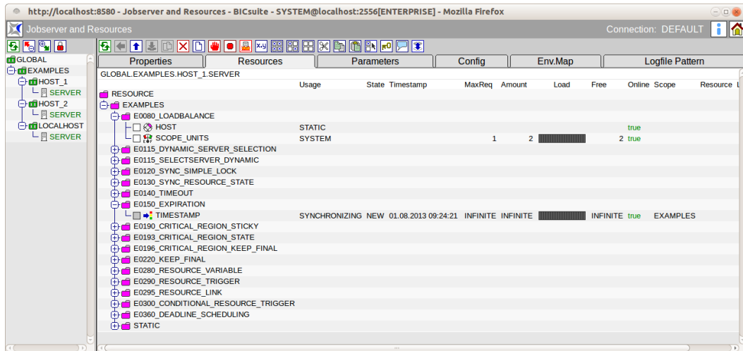
Figure 13.2: Job servers and Scope Navigator
