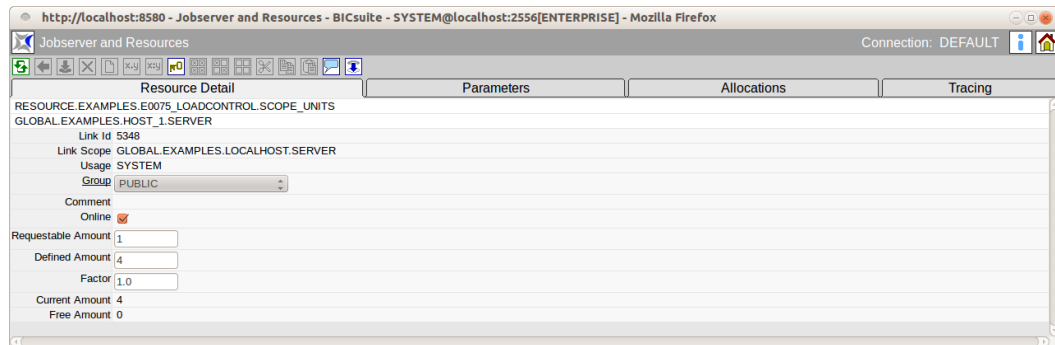
Figure 13.20: Information about a Resource Link
