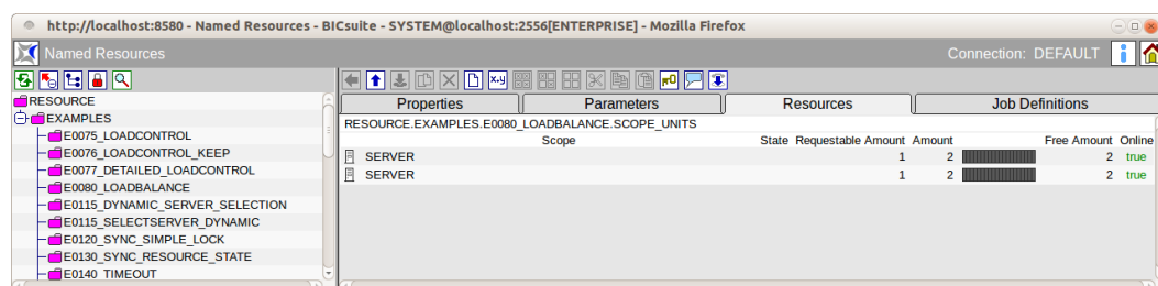
Figure 10.7: Named Resources; instances
