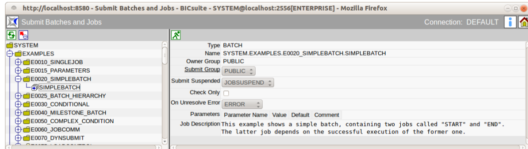
Figure 19.2: Submit navigation
