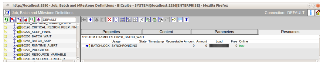
Figure 14.8: Folder resources
