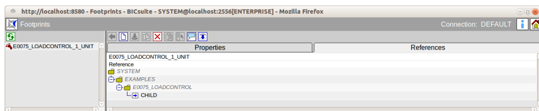
Figure 12.3: Footprint references
