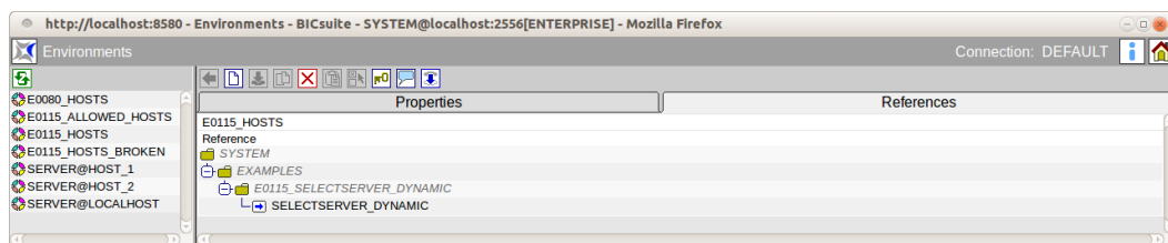
Figure 11.4: Environment references
