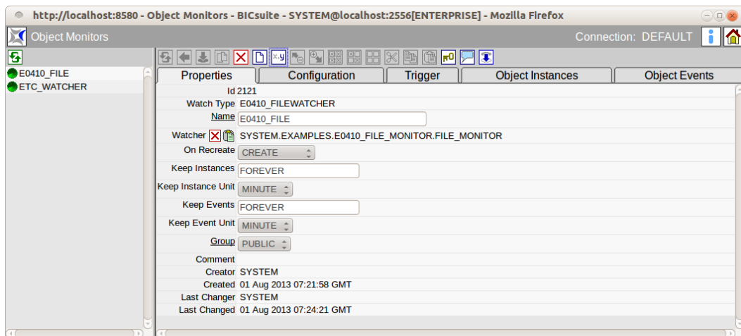
Figure 25.1: Object monitoring
