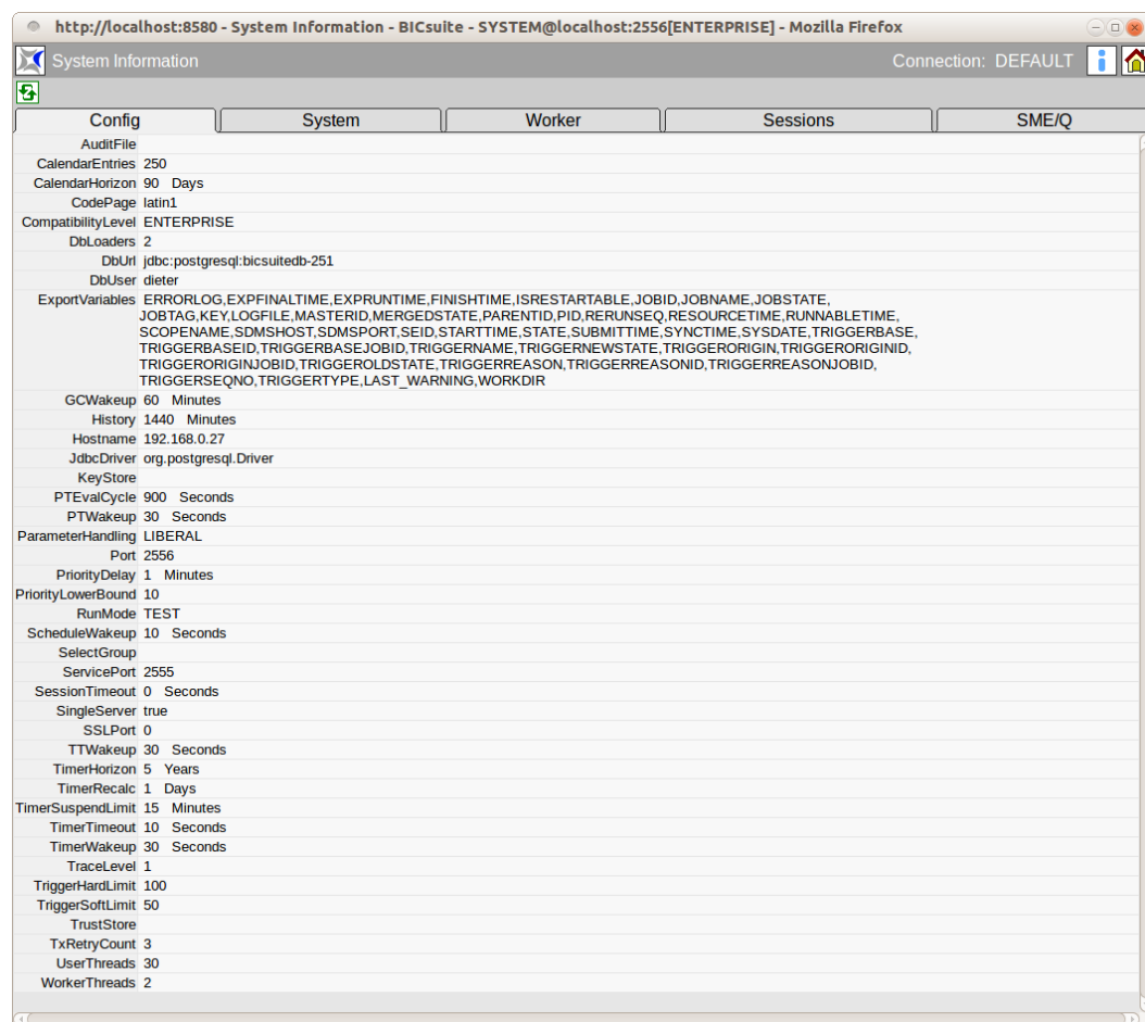
Figure 24.2: System configuration
