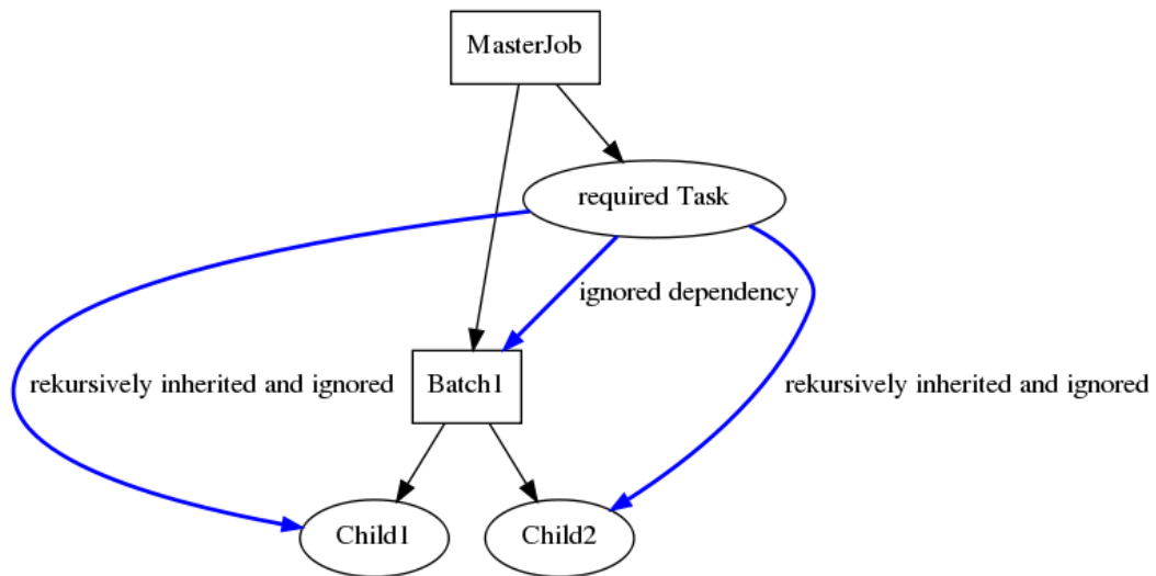
Figure 21.14: Example of a Recursive Ignore
