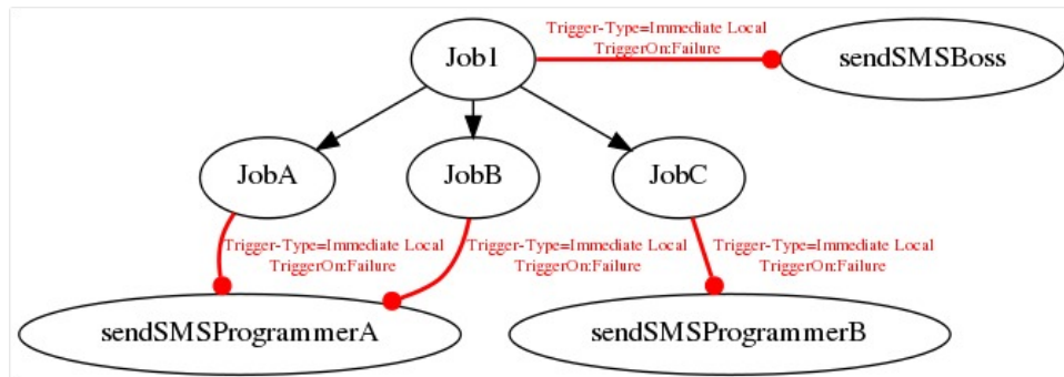
Figure 14.37: Example of an Immediate Local trigger
