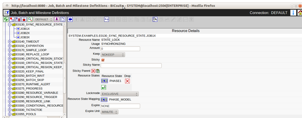
Figure 14.26: Batches and Jobs; Resource Requirement details
