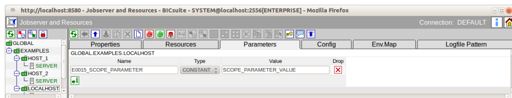
Figure 13.10: Job server and scope parameters
