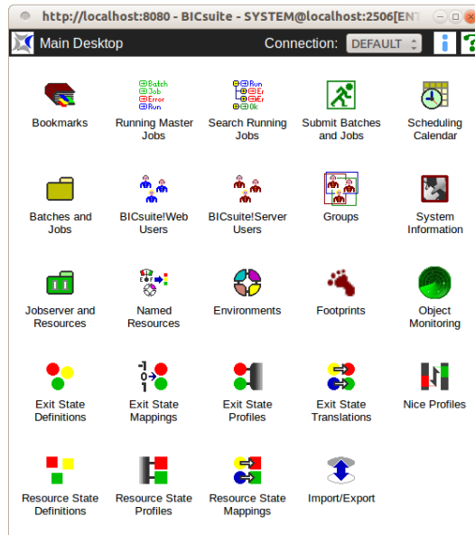
Figure 1.3: Main Desktop
