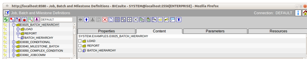
Figure 15.6: Folder content
