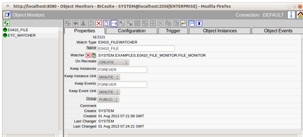
Figure 26.1: Object monitoring
