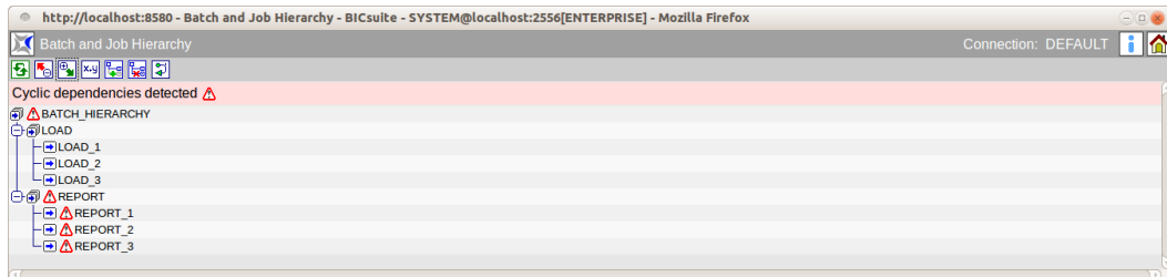
Figure 15.45: Cyclic dependencies
