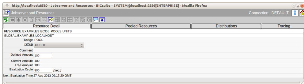
Figure 14.14: Pooled Resources
