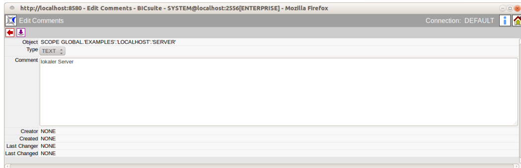
Figure 1.41: Recording comments
